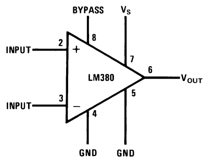
Figure 4. 8-Pin PDIP
