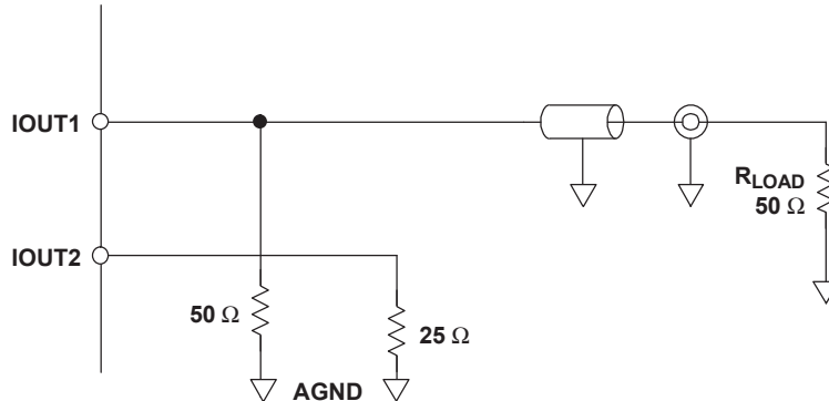
Figure 24. Driving a Doubly-Terminated 50-Ω Cable Using a Single-Ended Output
