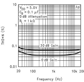
Mic Amplifier THD+N vs Frequency
