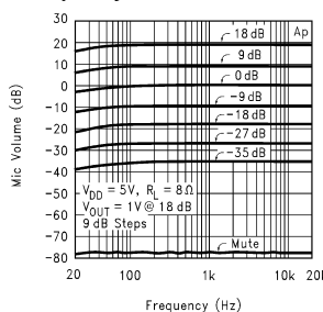
Mic Amplifier Attenuation vs Frequency
