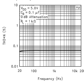
Loop-out THD+N vs Frequency
