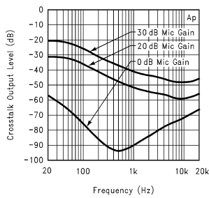
Mic Amplifier Crosstalk from Power Amplifier
