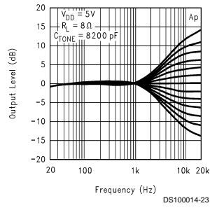
Treble Response vs Frequency
