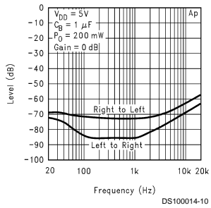
Power Amplifier Crosstalk
