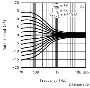
Bass Response vs Frequency
