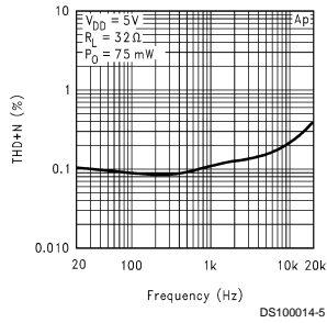
THD+N vs Frequency, 32Ω
