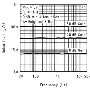
Mic Amplifier Noise Floor
