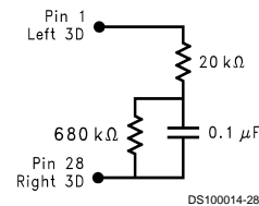
FIGURE 5. 3D Effect Components
