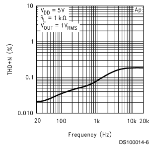
THD+N vs Frequency, 1 kΩ
