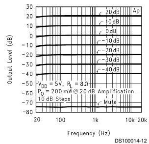
Power Amplifier Attenuation vs Frequency
