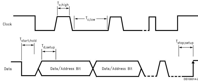
FIGURE 4. I 2 C Timing Diagram
