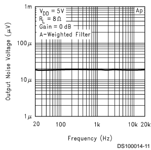
Power Amplifier Noise Floor
