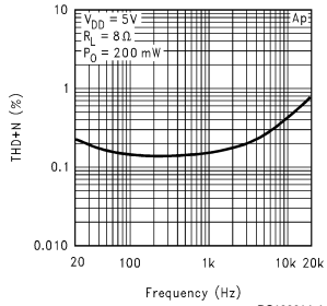
THD+N vs Frequency, 8Ω
