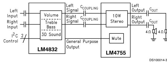
10W/ch System with I 2 C Controlled Tone, Volume and 3D Sound
