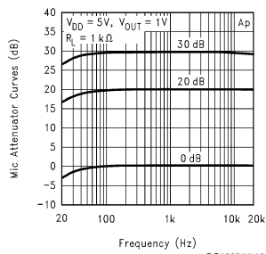
Mic Amplifier Gain vs Frequency
