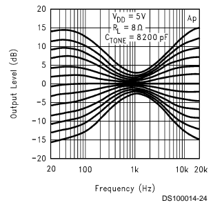
Bass and Treble Response vs Frequency
