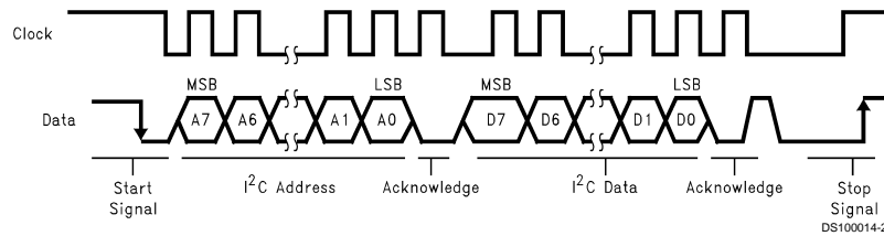
FIGURE 3. I 2 C Bus Format
