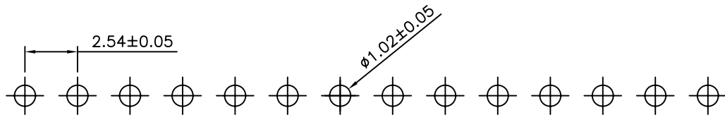
Recommended PCB Board Hole Layout
