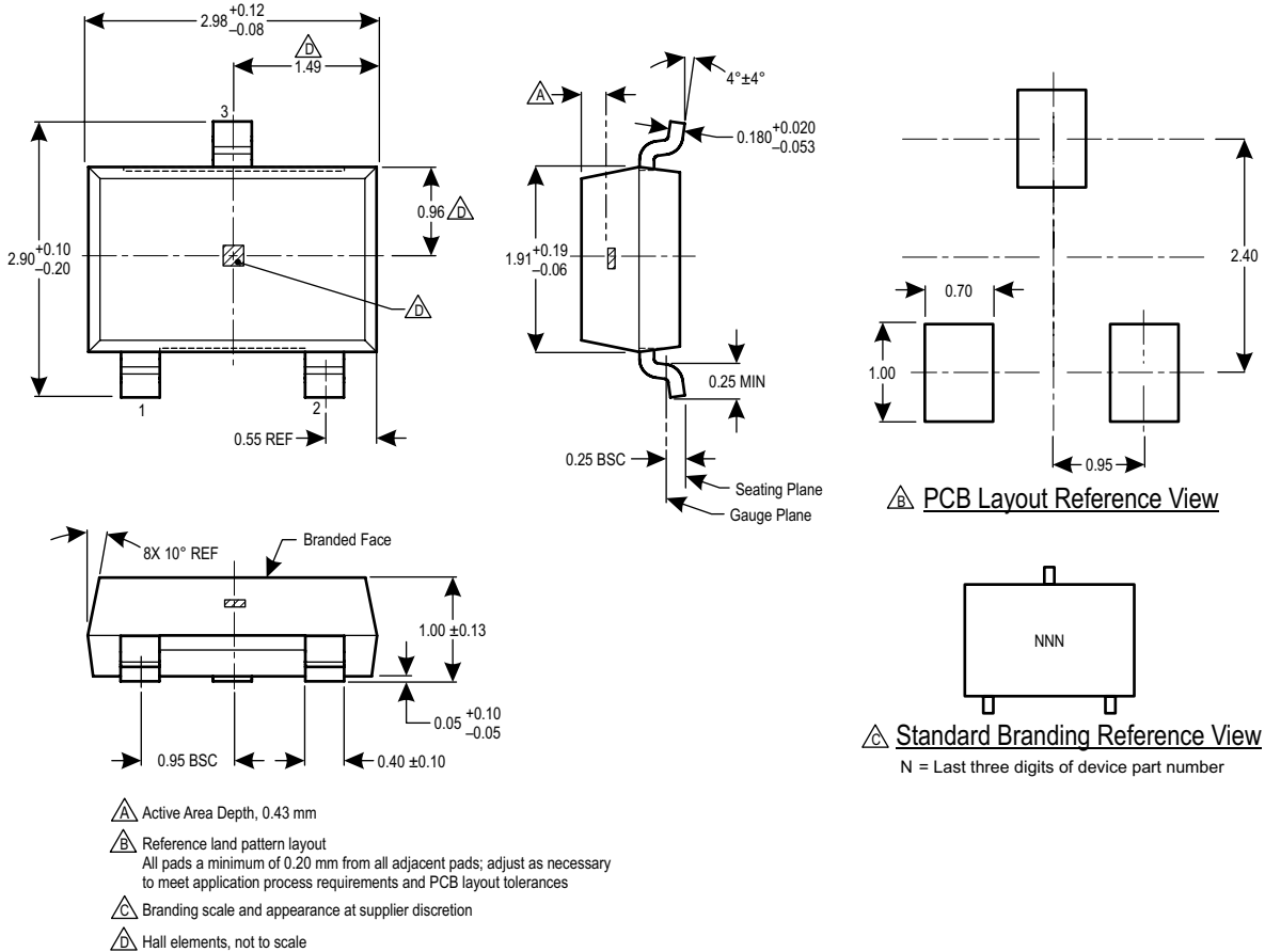
Figure 1: Package LH, 3-Pin; (SOT-23W)
