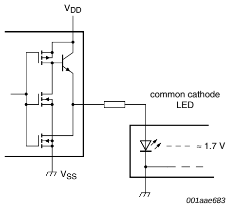
Fig 9. Connection to common cathode LED display readout
