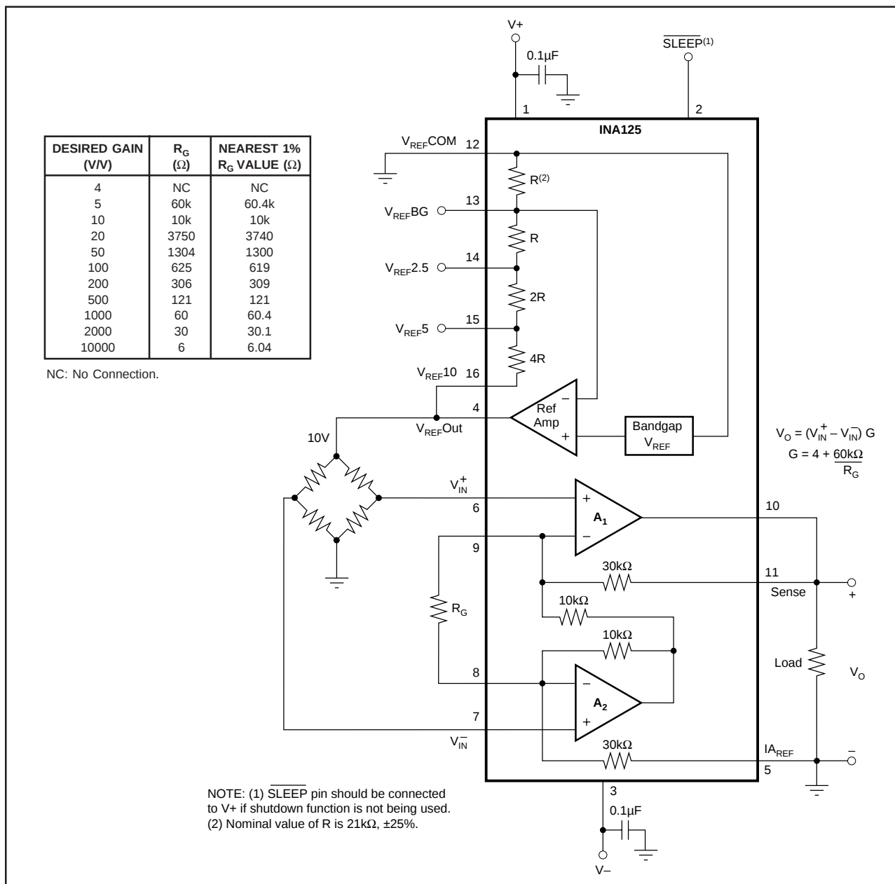
FIGURE 1. Basic Connections.
