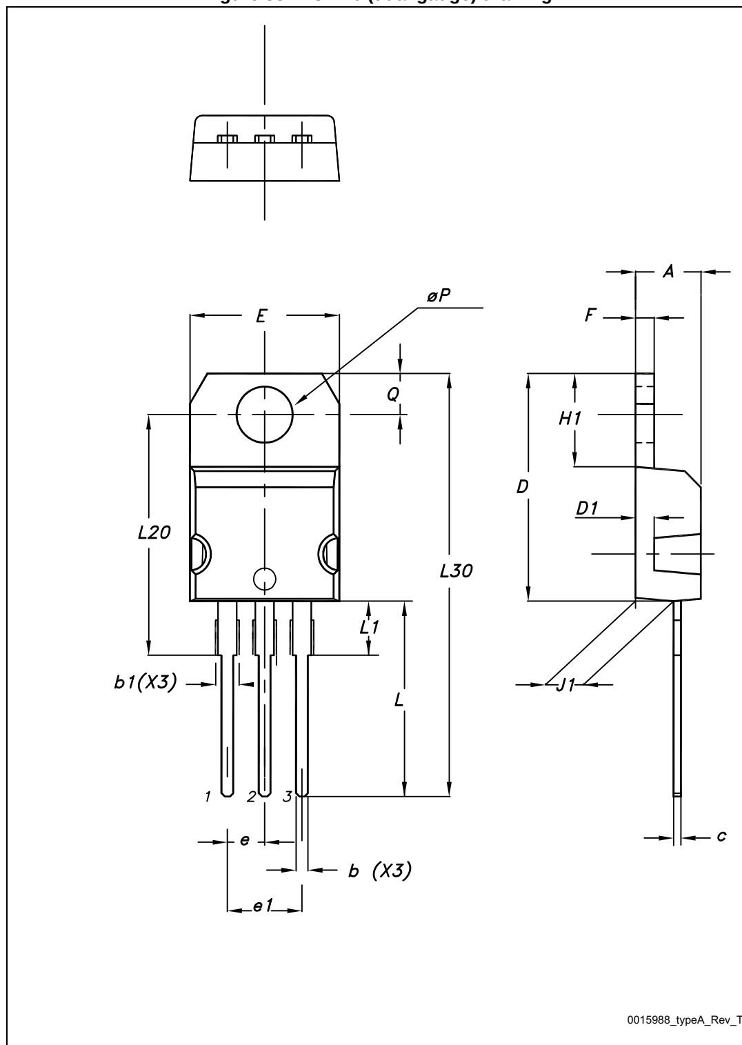
Figure 38. TO-220 (dual gauge) drawing
