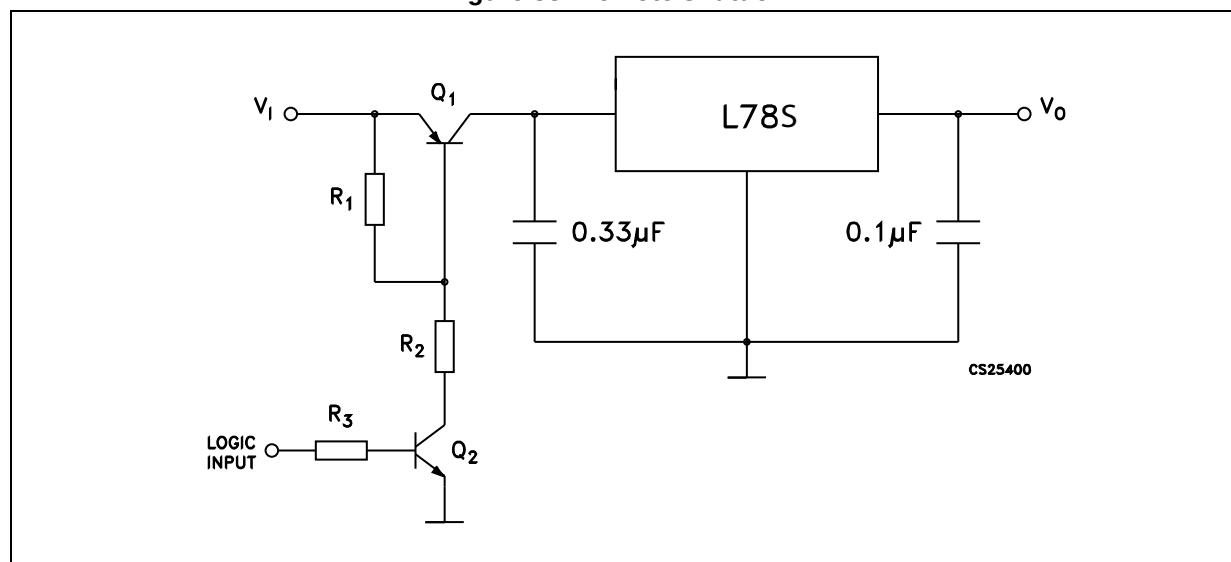
Figure 33. Remote shutdown
