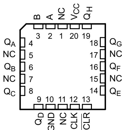
SN54HC164...FK PACKAGE (TOP VIEW)
