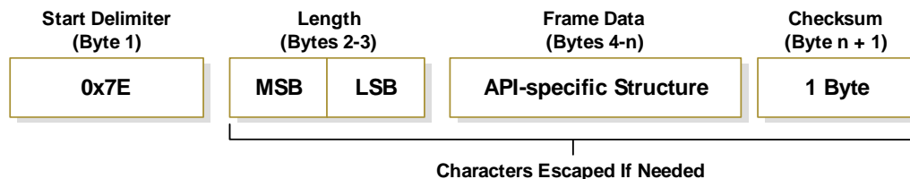
Figure 3-10. UART Data Frame Structure - with escape control characters:
