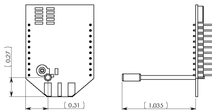
WIRE WHIP
